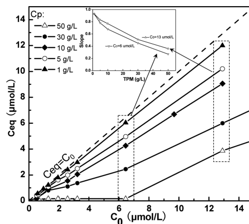
Figure 6. Relationship between the initial phosphate concentration ( C_0 ) and the final equilibrium concentration ( C_{\text{eq}} ) under different sediment concentrations (1, 5, 10, 30, and 50 g/L). The sediment sample came from Jinan station (H19). Dotted line represents a 1:1 slope between the C_0 and C_{\text{eq}} , meaning no adsorption occurs. The inserted chart describes the influence of TPM on the conservative behavior between the C_{\text{eq}} and C_0 .
