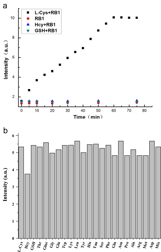
Fig. 6. (a) Time dependent fluorescence intensity changes of RB1 (10 \mu M) in the absence and presence of 20 eq. Cys, Hcy and GSH. (b) Fluorescence responses of RB1 (10 \mu M) solution at 552 nm to L-Cys and to the mixture of L-Cys with other bio-species; Mix = Hcy + GSH + Thr + Gluc + Gly + Trp + Lys + Leu + Try + His + Tau + Ser + Phe + Gln + Asn + Pro + Ala + Arg + Met + Asp, 200 \mu M respectively.
