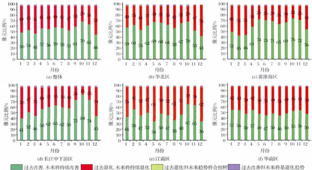
Fig. 2 Comparative characters of monthly NDVI variations
