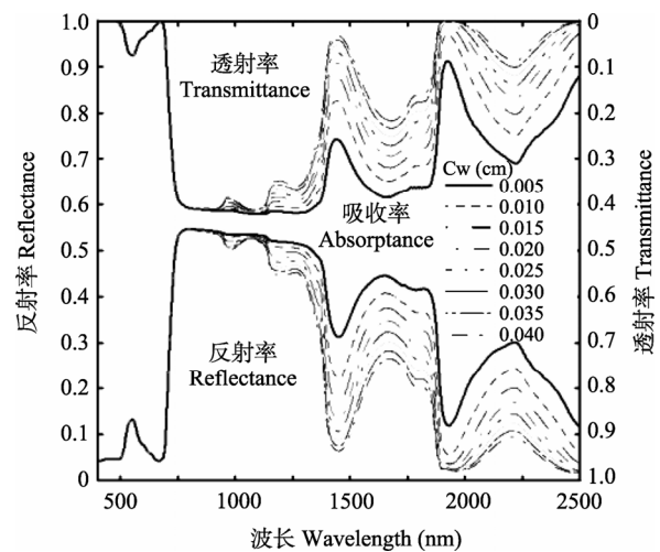
图 5 不同等效水厚条件下模拟的叶片光谱 Fig. 5 Simulated spectra of leaf under different equivalent water thickness
